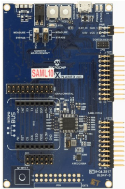
Microchip SAML10 Xplained Pro MCU: SAML10 (Cortex-M23)
