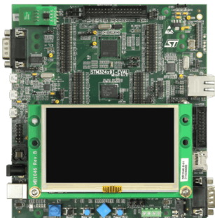
ST STM324x9I-EVAL MCU: STM32F429 (Cortex-M4)
